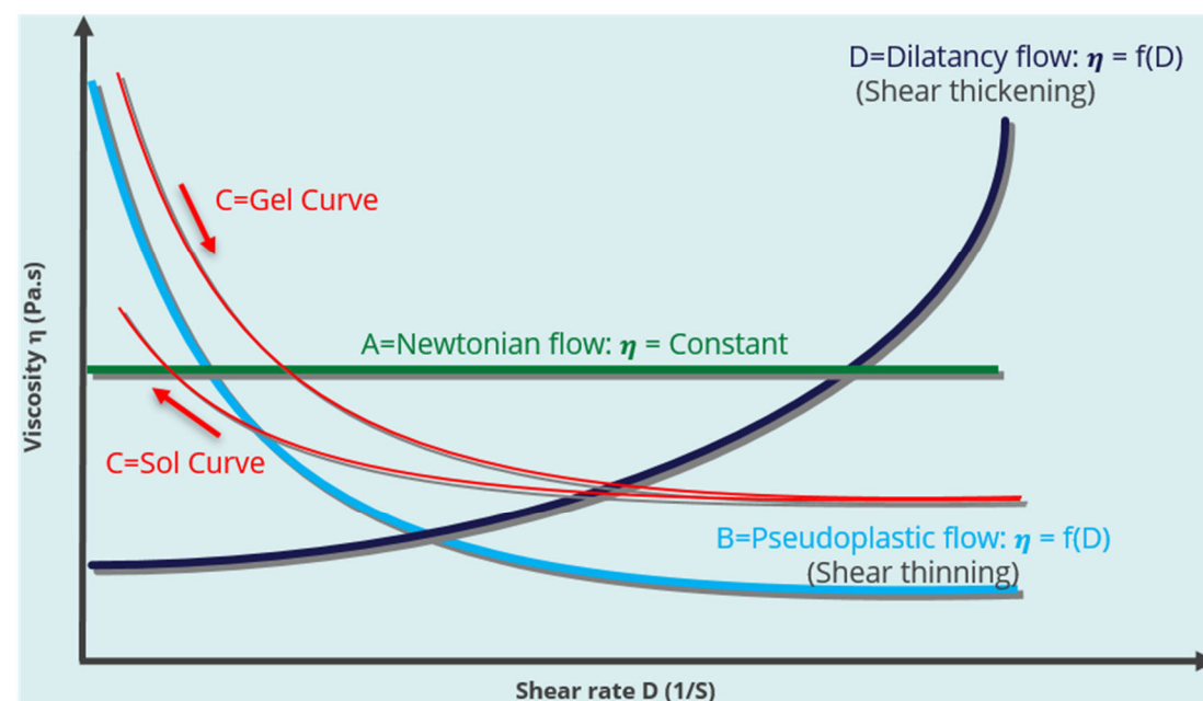
Viscosity curves and thixotropic flow
